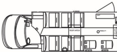
12 + 2 Passenger Collins Bus
